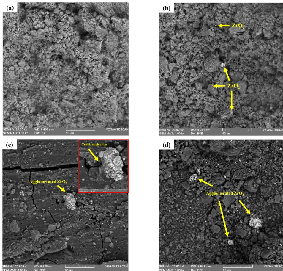
Fig. 7. SEM image of composites: a) Ca-Cement, b) 8\text{ZrO}_2\text{-Ca-Cement} , c) 10\text{ZrO}_2\text{-Ca-Cement} , d) 12\text{ZrO}_2\text{-Ca-Cement}
