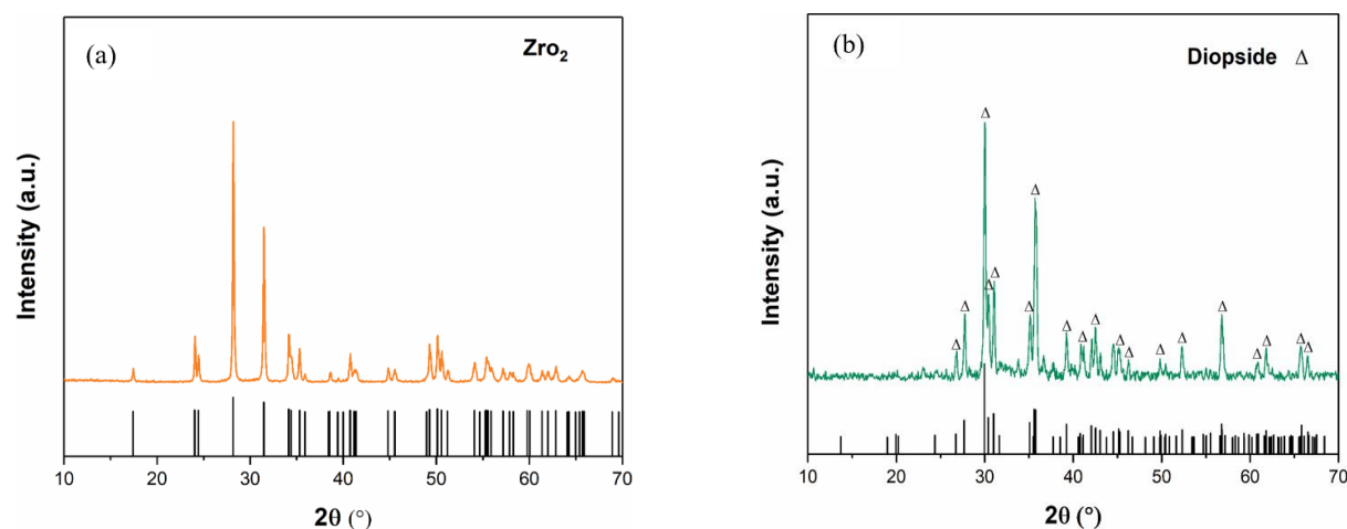
Fig. 2. XRD patterns of a) purchased zirconia ( ZrO_2 ) and b) synthesized diopside ( CaMgSi_2O_6 )
